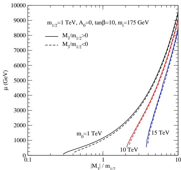
Figure 2: The values of \mu dictated by REWSB as a function of |M_3|/m_{1/2} , for A_0 = 0 , \tan \beta = 10 , \mu > 0 and m_t = 175 \text{ GeV} , at various values of m_0
