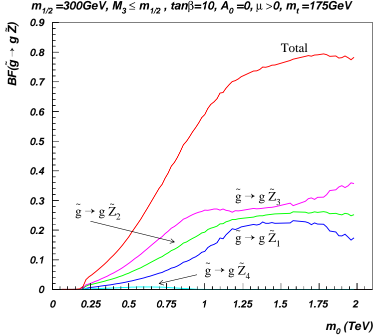
Figure 15: A plot of BF(\tilde{g} \rightarrow \tilde{Z}_i g) (for i = 1 - 4 ) versus m_0 for m_{1/2} = 300 GeV, A_0 = 0 , \tan\beta = 10 , \mu > 0 where at each point M_3 has been dialed so that \Omega_{\tilde{Z}_1} h^2 = 0.11 .
