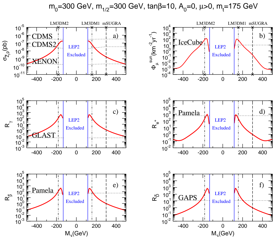
Figure 9: Rates for direct and indirect detection of neutralino dark matter vs. M_3 for m_0 = m_{1/2} = 300 \text{ GeV} , with \tan\beta = 10 , A_0 = 0 , \mu > 0 . Frames c) -f) show the ratio of indirect detection rates compared to the mSUGRA model. In this figure, we adopt the adiabatically contracted N03 distribution for halo dark matter for our projections of the reach of the various experiments.
