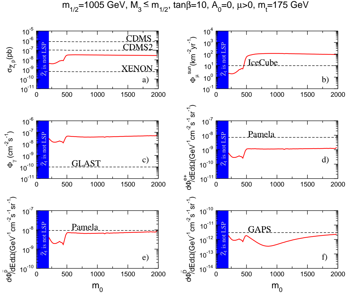
Figure 10: Rates for direct and indirect detection of neutralino dark matter vs. m_0 for the m_{1/2} = 1005 \text{ GeV} slice of the plane in figure 5b together with the projected sensitivities of the various experiments, assuming the adiabatically contracted N03 distribution for halo dark matter.
