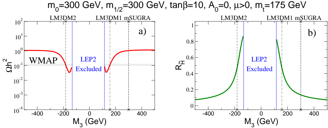
Figure 3: a) The neutralino relic density \Omega_{CDM} h^2 , and b) higgsino component R_{\tilde{H}} of the lightest neutralino as a function of M_3 for m_0 = 300 \text{ GeV} , m_{1/2} = 300 \text{ GeV} , A_0 = 0 , \tan\beta = 10 , \mu > 0 and m_t = 175 \text{ GeV} .
